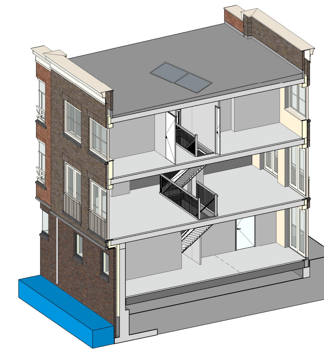
3D impressie
